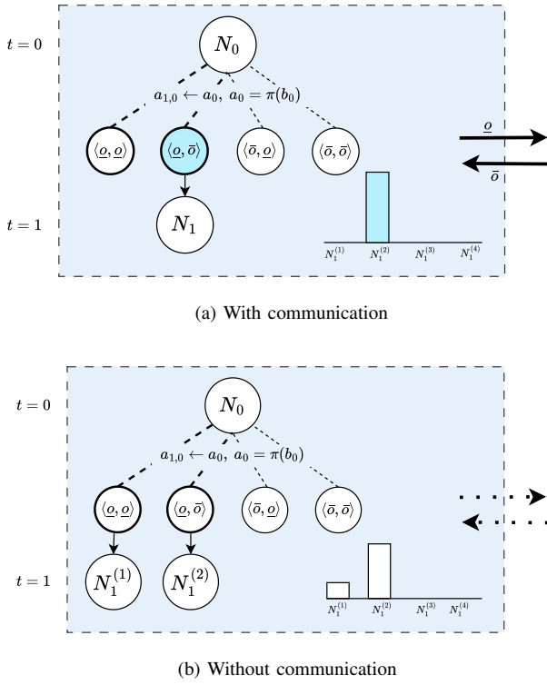
Fig. 3. Belief Space Propagation for the first time step, with and without communication, for a team of two agents. The perspective is that of Agent 1, executing local action a_{1,0} and receiving local observation o_{1,1} = \underline{o} .
