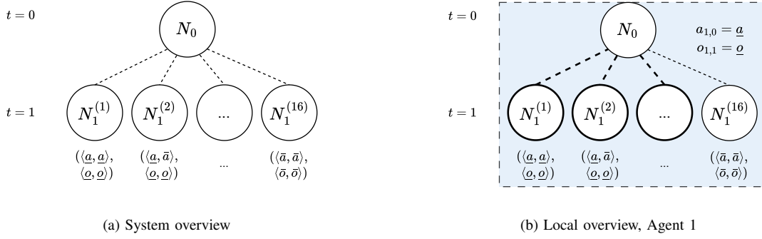
Fig. 2. Representation of the branching structure generated to account for all possible joint AOH. A common initial root N_0 represents the initial state of a system composed of two agents with local action and observation spaces A_i = \langle \underline{a}, \bar{a} \rangle , and O_i = \langle \underline{o}, \bar{o} \rangle , respectively, i = 1, 2 . On the left, all possible action-observation combinations (Fig. 2a). On the right, a local view of Agent 1 isolating the branches consistent with its own local AOH (Fig. 2b).
